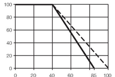
Derating curve of a filter (simplified). Diagram: permitted operating current in % I_n vs ambient temperature
